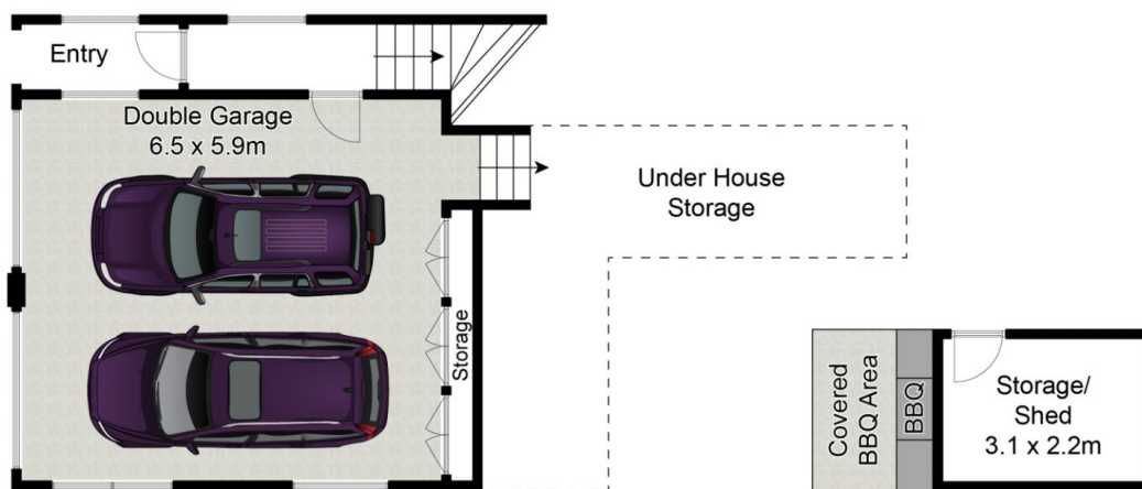
Entry Level
